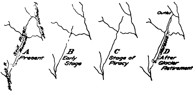
FIG. 367. — Diagrams to illustrate the episodes in the recent history of the Still River tributary to the Farmington in Connecticut. A, present drainage; B, early stage; C, after capture of a tributary to the Farmington; D, after blocking by morainal obstructions of the ice age.
